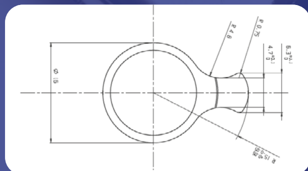
Lever "UNI"
