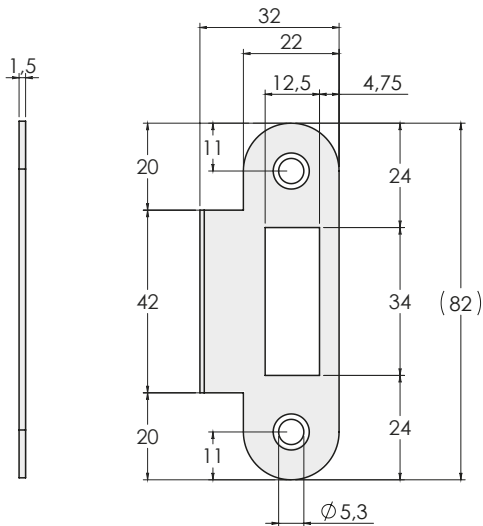
reversibile per profili in alluminio | Art. W120 reversible for aluminium / PVC frames
