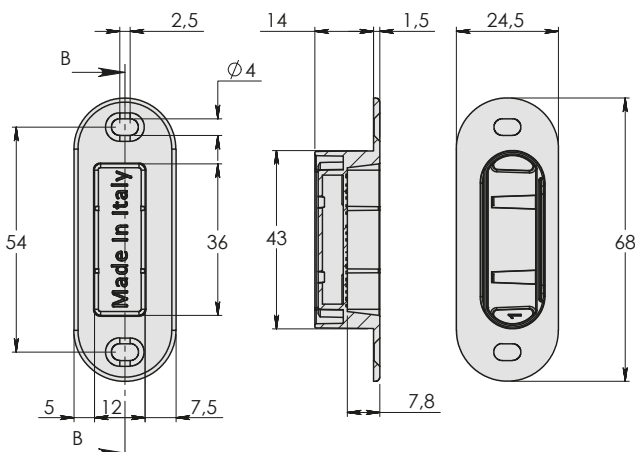
reversibile per profili in alluminio | Art. W120 reversible for aluminium / PVC frames
